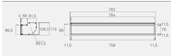
C4000 Difusor entrada practicable
