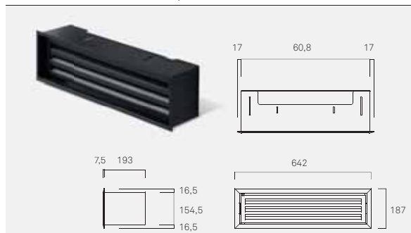
C4000 Difusor entrada practicable
